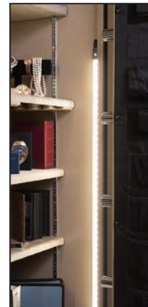
36" LED LIGHT KIT Has two 36" light strips with high-intensity white LED lights and a motion sensor that automatically turns the lights on when motion is detected. The lights turn off 30 seconds after motion has stopped. This light kit can be installed on any AMSEC safe and is also available as a retrofit kit.
